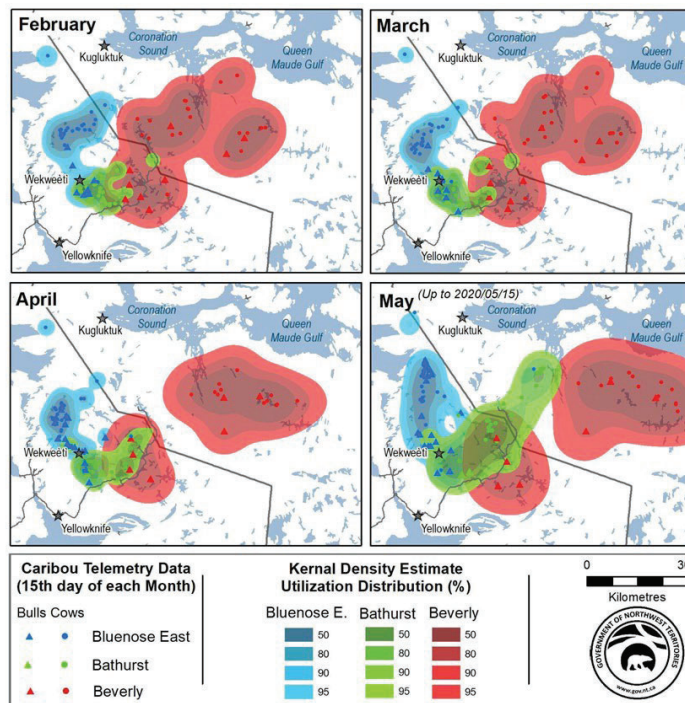
Figure 4. Monthly UDs from 2020 for Bathurst, Bluenose-East and Beverly caribou herds based on KDE. Adapted from Nishi et al. 2020.
