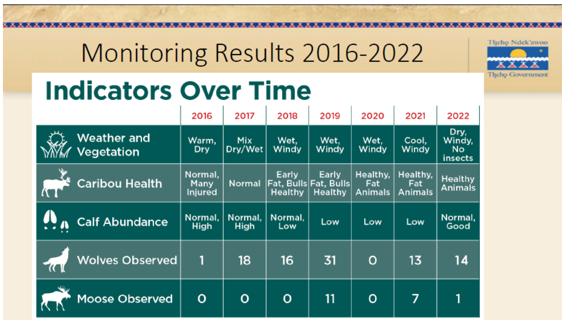
Figure 49. Summary of monitoring of Bathurst caribou (Kokètì Ekwò) in the Contwoyto Lake area (Kokètì) from the Ekwò Nàxoèdee K'è caribou monitoring carried out by the Tłıchǫ Government. Courtesy of P. Jacobsen, Tłıchǫ Government.
